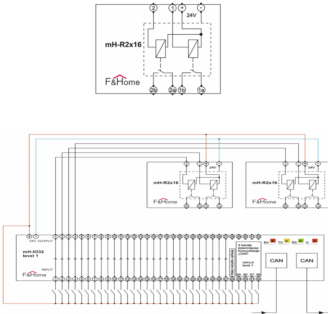
Connecting the actuator module (relays - mH-R2x16) to the input-output module.
